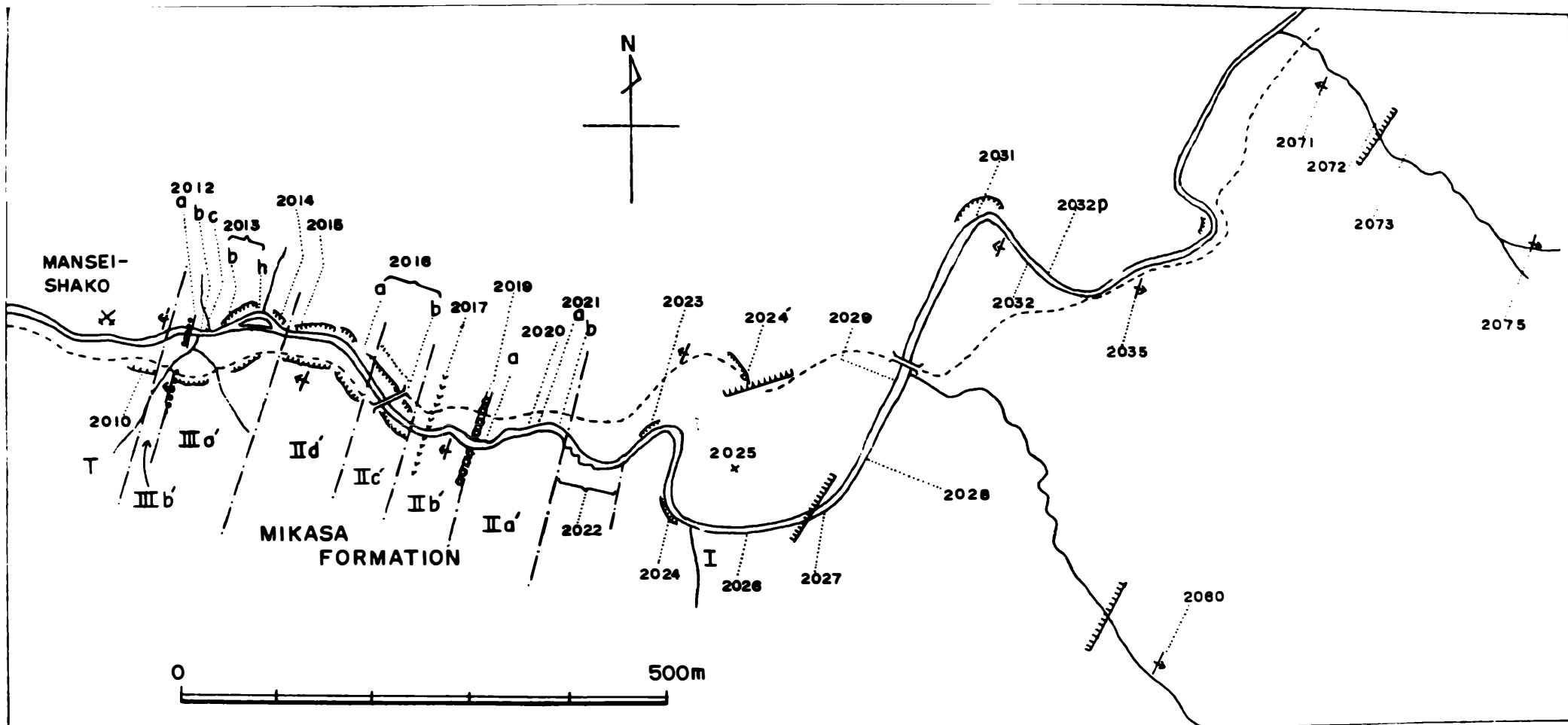
Fig. 3. Route map along the Pombets, a tributary of the Ikushumbets. All the fossil localities should have the prefix Ik. For the abbreviations of the stratigraphic subdivisions (e. g. IIa', IIb', etc.) see Fig. 5.
