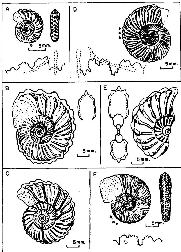
Fig. 6. Diagram showing immature shells of highly plastic Collignoniceratidae woollgari (MANTELL). Figures are drawn on the basis of the representative specimens, from loc. TM. 31, 2 miles southwest of New Castle, Wyoming, as indicated below, sometimes slightly restored. (See also Plates 1-3). A: GK. H7504 of Group A, in which the woollgari type coarse ornament appears very early in ontogeny; B: GK. H7447 of Group B, which can be regarded as the most typical representative of C. woollgari ; C: GK. H7495, of Group C, which is characterized by ribs of unequal intensity, foreshadowing Prionocyclus hyatti ; D: GK. H7496 of Group D, characterized by the persistency of crowded, fine ribs with two ventrolateral tubercles, resembling C. woollgari bakeri ; E: GK. H7453 of Group E, which has regularly and gradually distant ribs and a subrectangular whorl-section, foreshadowing Subprionocyclus branneri ; F: GK. H7494, which is characterized by dense, fine, flexuous, often branching and inserted ribs with late appearing inner ventrolateral tubercles, foreshadowing Subprionocyclus hitchinensis or immature S. neptuni . (T. M. delin.)
