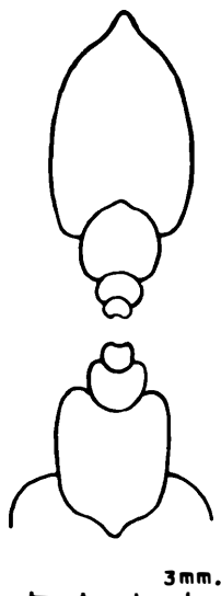
Fig. 12. Lymaniceras planulatum sp. nov. Cross section of an immature specimen, GK. H5467b, from loc. Ik2012c, showing the ontogenetic change in whorl shape. (T. M. delin.)
