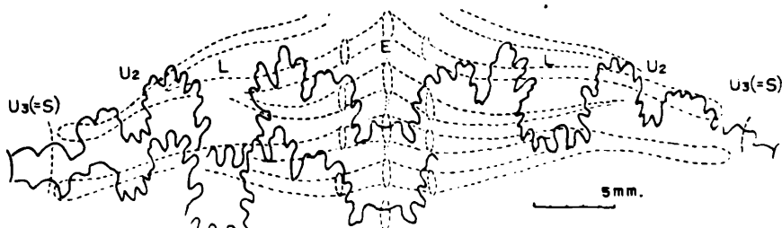
Fig. 36. Reesidites minimus (HAYASAKA and FUKADA). Last two external sutures at whorl-height = c. 15 mm. in GK. H4089, a specimen smaller than the holotype, from loc. 1k2013b, Pombets. The suture is not strictly symmetric between left and right sides. (T. M. delin.)
