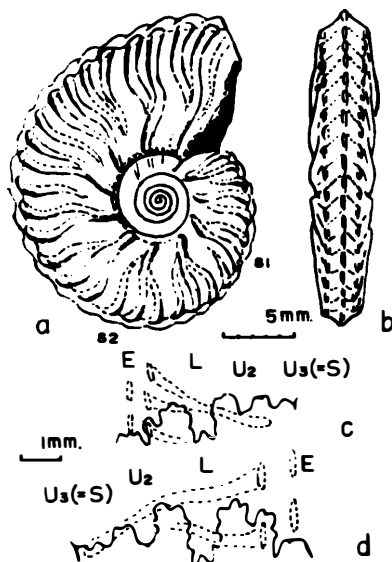
Fig. 37. Reesidites minimus (HAYASAKA and FUKADA). An example of the immature shell, GK. H4024, from loc. Ik946, Ikushumbets. Diagrammatic sketches in (a) lateral and (b) ventral views; (c) suture at s_1 ; (d) suture at s_2 in Fig. a.
