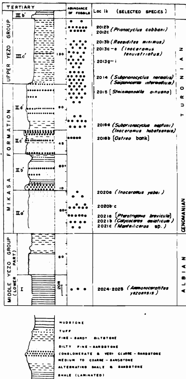
Fig. 5. Columnar section showing the stratigraphic sequence of the Cretaceous sediments along the Pombets. See Fig. 3 for the fossil localities. Lithologic symbols at the bottom. (in IIIa'): Fault.
