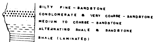
Fig. 5. Columnar section showing the stratigraphic sequence of the Cretaceous sediments along the Pombets. See Fig. 3 for the fossil localities. Lithologic symbols at the bottom. (in IIIa') : Fault.
