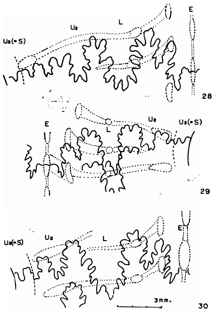
Figs. 28-30. Subprinocyclus normalis (ANDERSON). External sutures, showing the disposition of ribs, tubercles and ventral keel with dotted lines.
