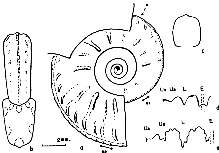
Fig. 14. Lymaniceras planulatum sp. nov. Early immature shell in the nuclear part of GK. H5429a, from loc. Ik2012c, Pombets. (a) Side view; (b) front view; (c) diagrammatic whorl section at q of Fig. a; (d, e) external sutures at s_1 and s_2 in Fig. a. (T.M. delin.)
