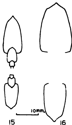
Figs. 15, 16. Lymaniceras planulatum sp. nov.
