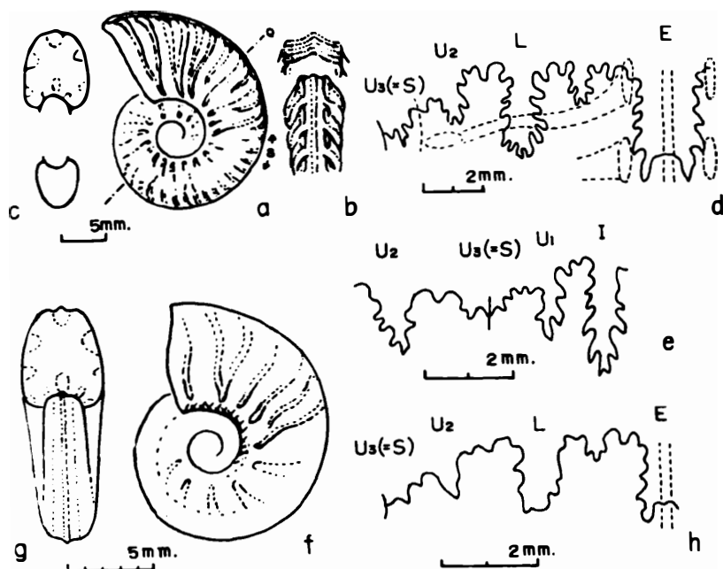
Fig. 40. Niceforoceras (?) japonicum sp. nov. Holotype GK.115495, from loc. JPE. 12. Kumaoui-zawa, Ikushumbetsu, diagrammatic sketches. (a) Lateral view; (b) part of venter; (c) whorl-section at a in Fig. (a); (d) external suture at whorl-height=7 mm.; (e) internal suture at almost the same stage; (f) inner whorl in lateral view; (g) inner whorl in frontal view; (h) external suture of the inner whorl.
