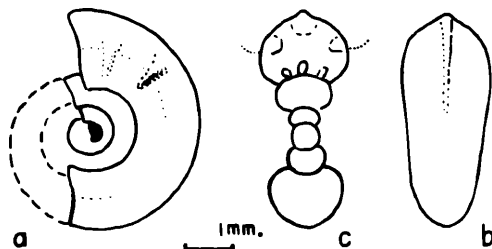
Fig. 13. Lymaniceras planulatum sp. nov. Inner nuclear part of GK. H5527, from loc. B223, Bibai. (a) Lateral and (b) ventral views; (c) cross section. (T. M. delin.)
