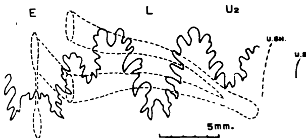
Fig. 35. Reesidites minimus (HAYASAKA and FUKADA). GK. H4090. a topotype nearly as large as the holotype. The last fifth suture at whorl-height = c. 25 mm. (T. M. delin.)
