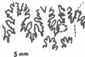
Fig. 6. Urakawites rotalinoides (YABE). External suture-line of lectotype, IGPS. 54438, in the middle growth-stage.
