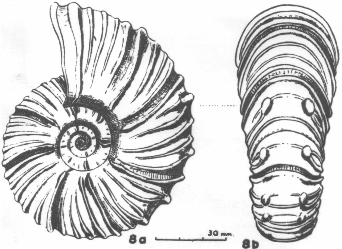
Fig. 8. Teshioites ryugasensis sp. nov. Lateral (a) and ventral (b) views of the adult shell, synthetized illustration.
