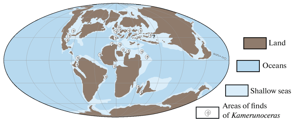
Fig. 4. Scheme of geographical distribution of Kamerunoceras turoniense (d'Orb.) on a paleogeographic basis (after R. Blakey, with changes).
