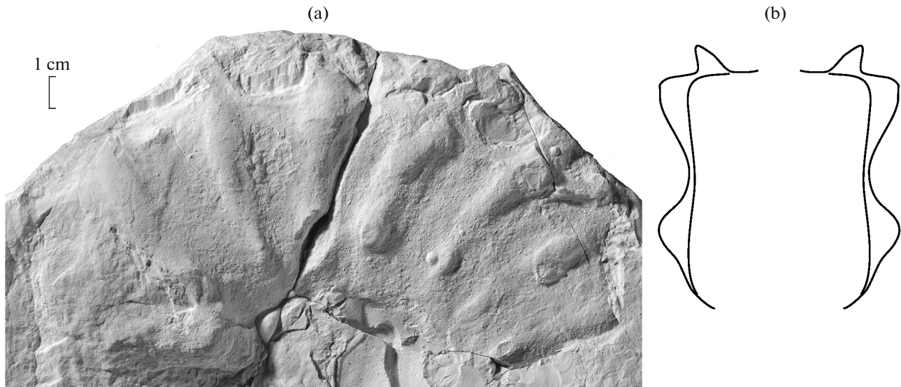
Fig. 3. Kamerunoceras sp. ex gr. turoniense (d'Orb.), specimen no. 149/7: (a) lateral view, (b) reconstructed section of the shell through the main ribs; lower Turonian, Member IX, Aksu-Dere ravine, Bakhchisaray district, Republic of Crimea. Collected by Fokin, 2023. The specimen is covered with ammonium chloride. Photograph by E.Yu. Baraboshkin.
