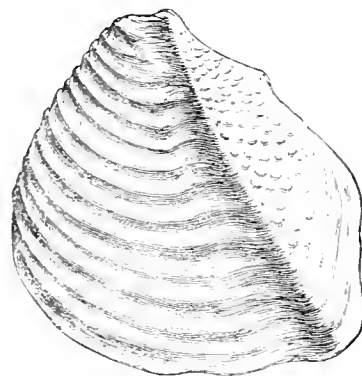
Trigonion Moorei , Lyc. Western Australia.
