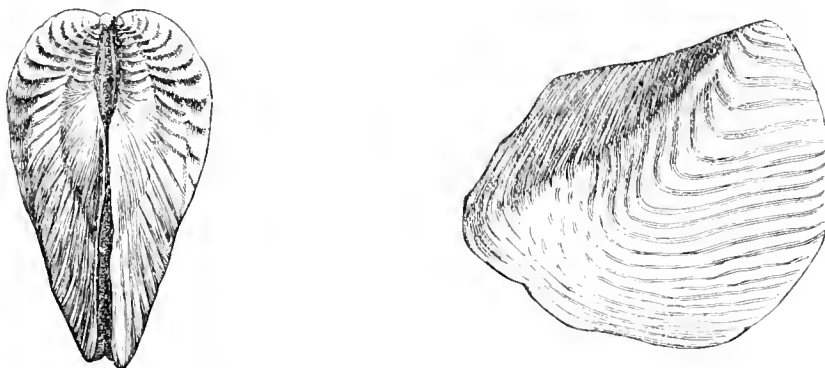
Trigonía undulata , From. Locality, the Lebanon east of Beyrout.
