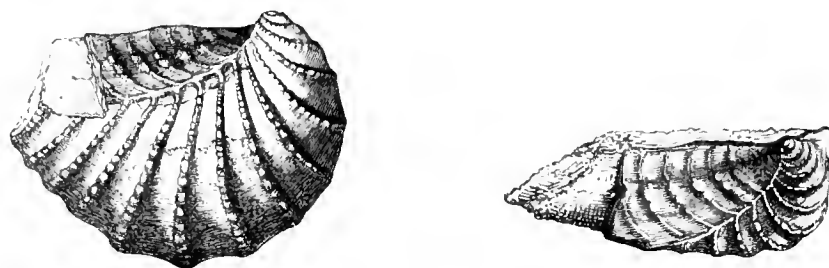
Trigonia Forbesii , Lycett, from Verdachellum, India.
