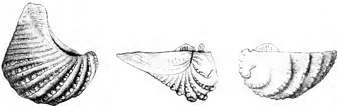
Three views of the valves of Trigonionia ventricosa , Krauss, from South Africa.
