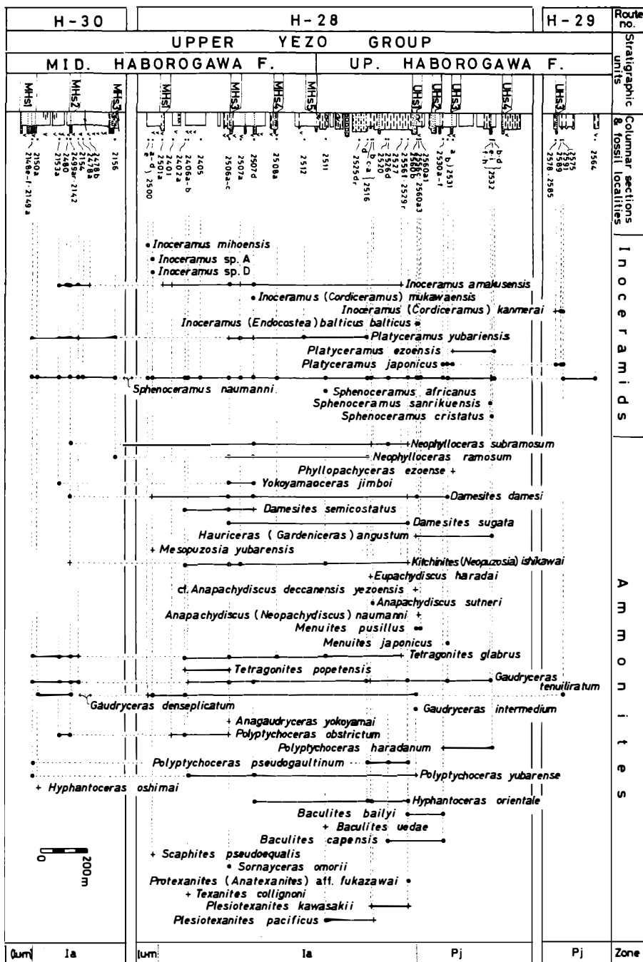
Fig. 9. Biostratigraphic successions of the Upper Yezo Group along the Nakanofutamata-gawa in the Haboro area, Hokkaido. Route numbers are shown in Figs. 2, 3. Put prefix RH on each loc. no.
