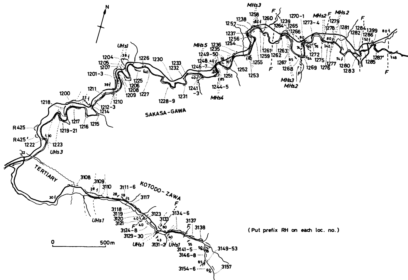
Fig. 18. Route map along the Sakasa-gawa in the Haboro area.
