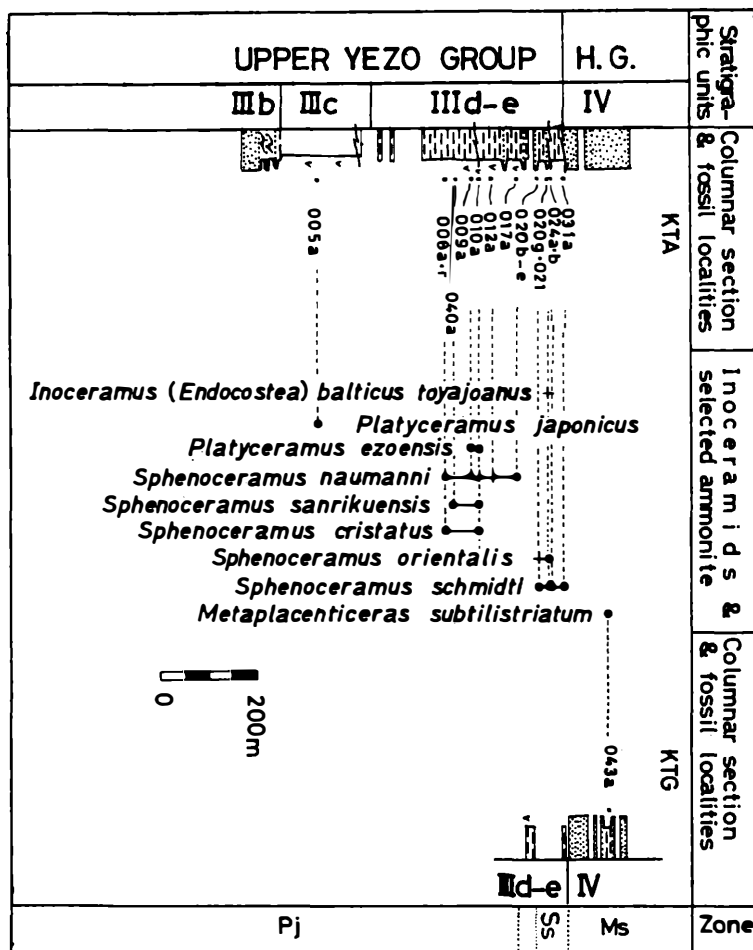
Fig. 4a. Biostratigraphic successions of the Upper Yezo Group and the Hako-buchi Group along the Tanno-sawa (left column) and Gakkono-sawa (right column) in the Saku area, Hokkaido. Legend is shown in Fig. 7. Stratigraphic units are after MATSUMOTO (1942b).
