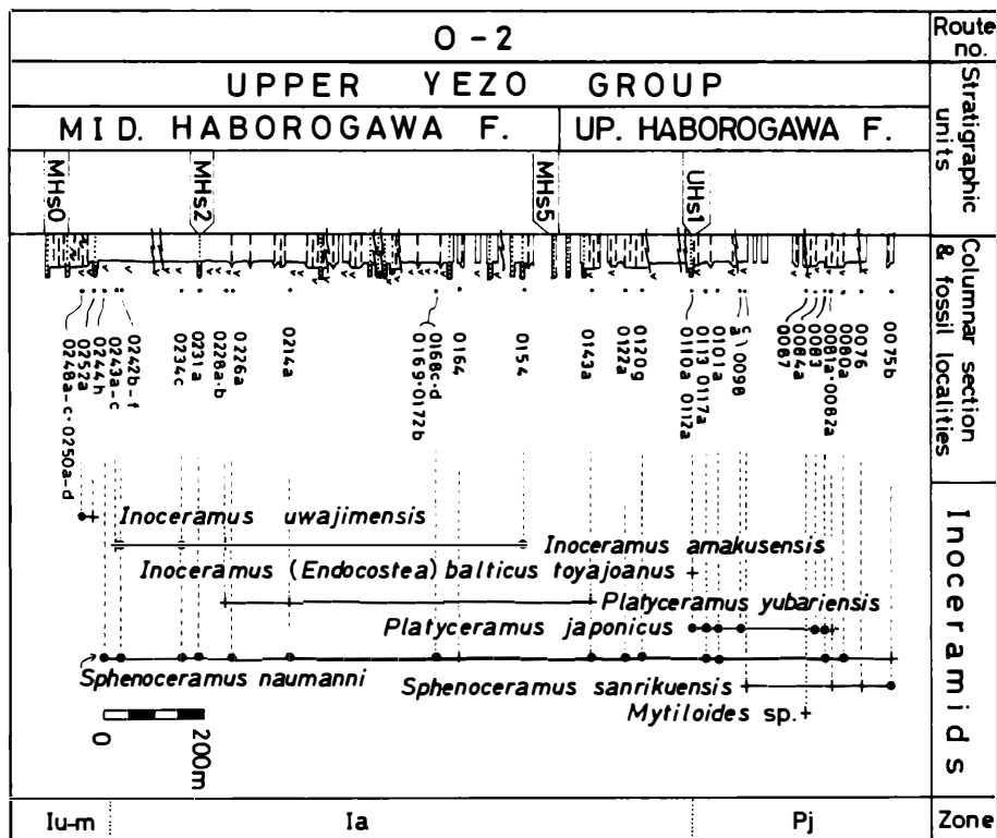
Fig. 15b. Biostratigraphic successions of the Upper Yezo Group along the Akano-sawa in the Obira area, Hokkaido. Route number is shown in Figs. 2, 3. Put prefix RO on each loc. no.
