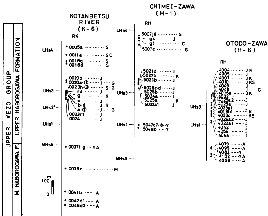
Fig. 5. Stratigraphic relationships between the selected mega- and micro-fossils, along the Otodo-zawa, Chimei-zawa and Kotanbetsu River.
