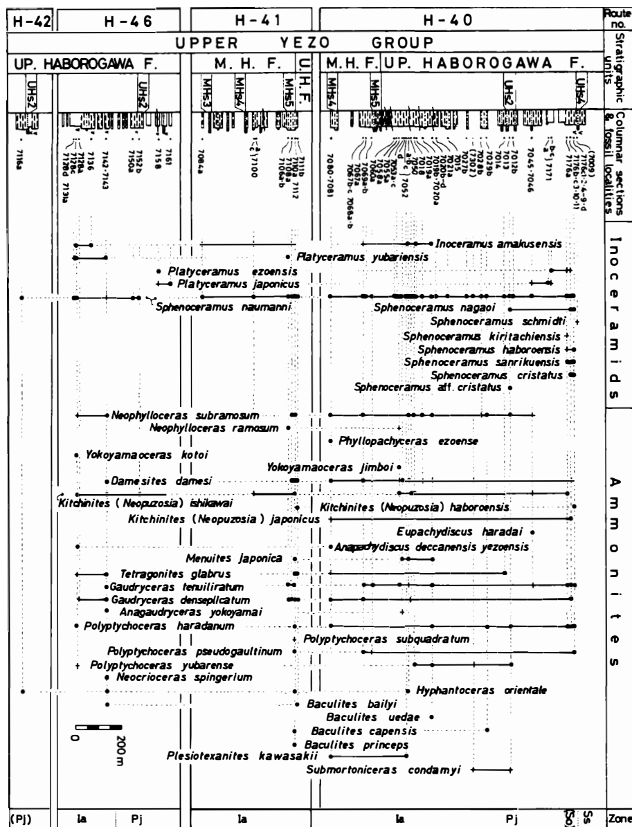
Fig. 8. Biostratigraphic successions of the Upper Yezo Group along the Deto-futamataga-gawa in the Haboro area, Hokkaido. Route numbers are shown in Figs. 2, 3. Numbers in parentheses show inferred horizon from the neighbouring route. Put prefix RH on each loc. no.
