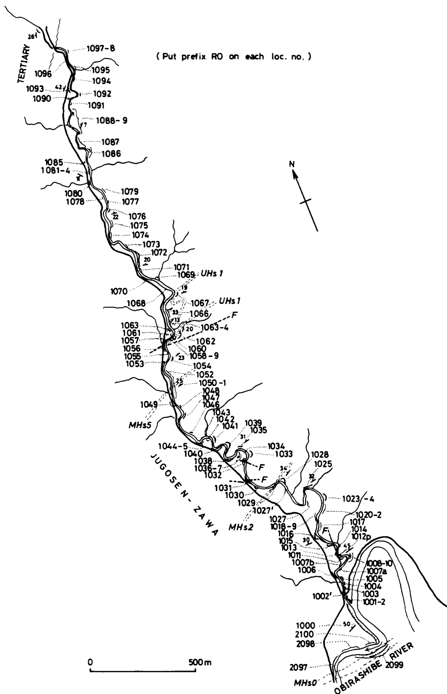
Fig. 26. Route map along the Jugosen-zawa in the Obira area.
