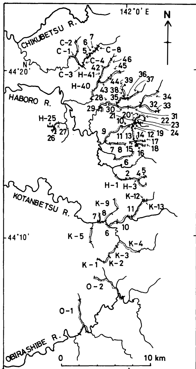
Fig. 2. Index map of the Chikubetsu, Haboro, Kotanbetsu and Obira areas indicating the routes C-1 to O-2 along which the Cretaceous sequences were measured and illustrated in Fig. 3.
